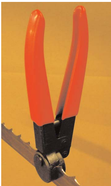
Blade Handsetter TS-101: Not Adjustable
